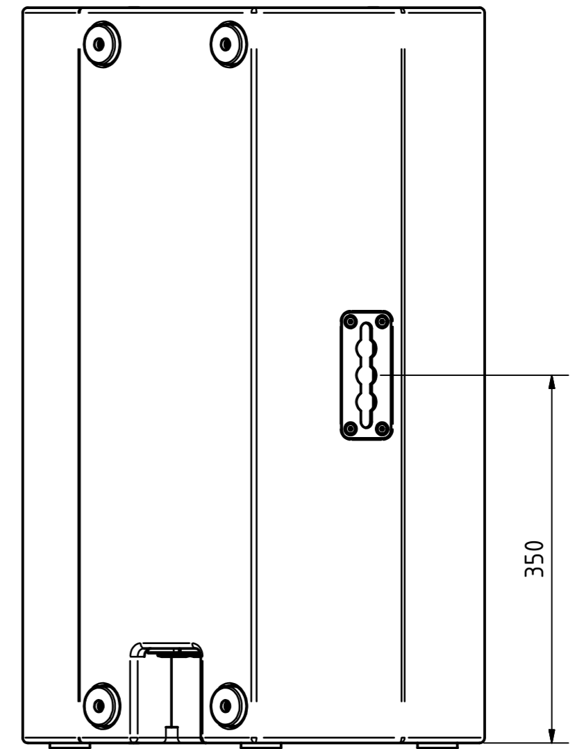
rear view
